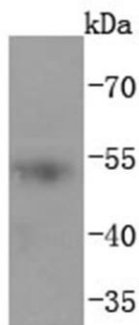
Fig. 1. Western blot analysis of Acetyl-p53 (Lys382) on human skin lysates using anti-Acetyl-p53 (Lys382) antibody at 1/1,000 dilution.
