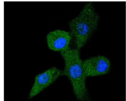
Fig. 2. ICC staining Acetyl-p53 (Lys382) in A549 cells (green). The nuclear counter stain is DAPI (blue). Cells were fixed in paraformaldehyde, permeabilised with 0.25% Triton X-100/PBS.
