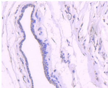
Fig. 3. Immunohistochemical analysis of paraffin-embedded human breast carcinoma tissue using anti-Acetyl-p53 (Lys382) antibody. Counter stained with hematoxylin.
